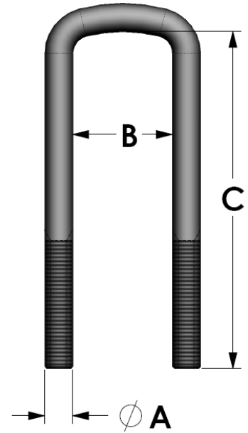
SEMI-ROUND BEND
