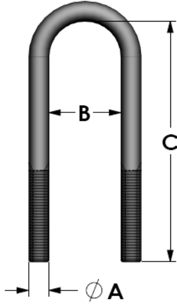
ROUND BEND
