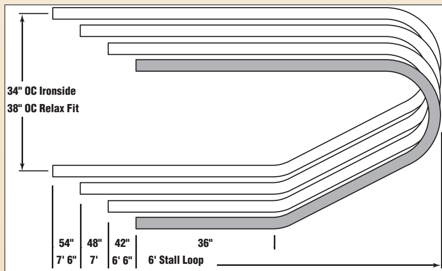
New! Ironside Head to Head Stall System with Weld-free Clamp System
