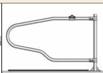
New! Relax Fit Single Stall System with Weld-free Clamp System
