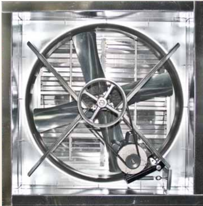
Heavy duty X-frame motor mount (Shown without rear guard for illustration purposes only)
